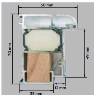
CROSS-SECTION OF TERMO FRAME
