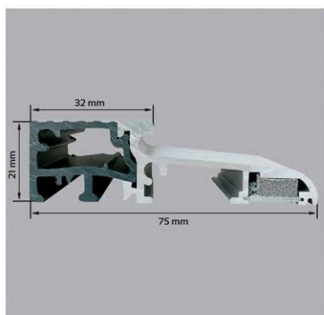
ENERGO THRESHOLD WITH THERMAL INSERT
