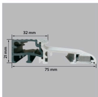
ENERGO THRESHOLD WITH THERMAL INSERT
