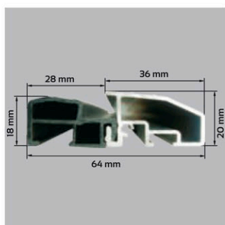
THRESHOLD WITH THERMAL INSERT
