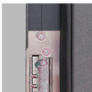
LATCH ADJUSTMENT
