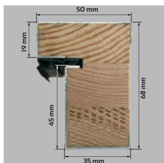
CROSS-SECTION OF ENERGO FRAME
