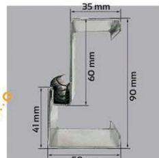
CROSS-SECTION OF SYMMETRICAL FRAME WITH SEAL
