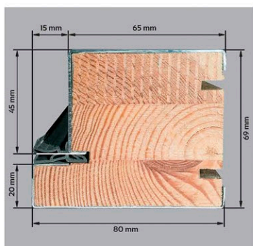
CROSS-SECTION OF ENERGO FRAME
