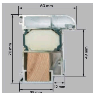
TERMO FRAME CROSS SECTION
